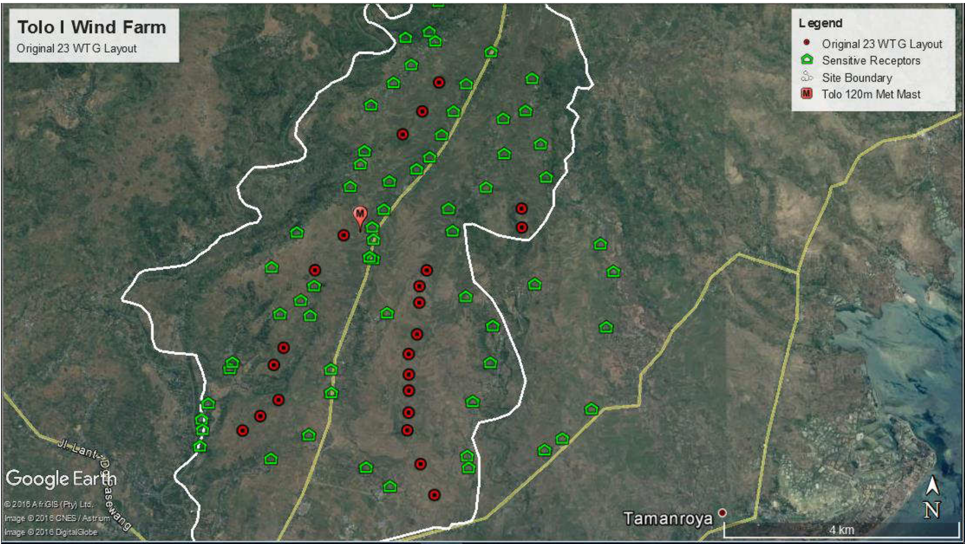
12. Original 23 turbine layout with sensitive receptors
